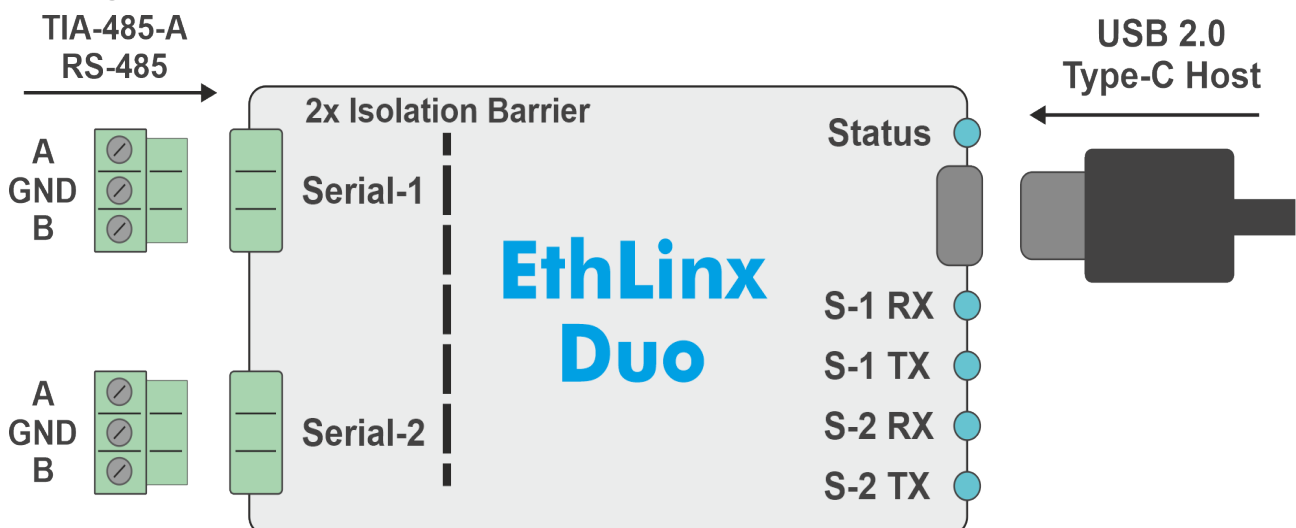
Image 1: Basic Wiring Diagram with serial connections and LED description, EthLinx Duo
